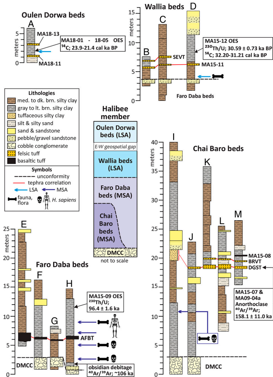
Fig. 2. Halibee member litho- and chronostratigraphy. Measured sections representative of the OUD (A), Wallia (B–D), Faro Daba (E–H), and Chai Baro (I–M) beds are illustrated, with letters corresponding to locations plotted in Fig. 1. A central schematic composite section summarizes the relationships between these beds. Important marker horizons and the stratigraphic levels of chronologic results and archaeological and paleontological resources are indicated. Photographs of outcrops on which these sections are based are presented in SI Appendix . Descriptions and discussions of the materials and methods used for geochronologic determinations and of the tephra and their chemical signatures are contained in the main text and SI Appendix . A more detailed presentation of the age determinations is summarized in Fig. 3.
